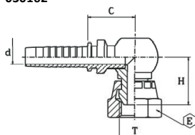
BSP COMPACT FEMALE 60° FLARE 90° ELBOW FEMMINA COMPATTA 90° BSP SV.60° 030162
