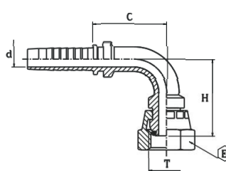
BSP FEMALE 60° FLARE 90° ELBOW WITH O'RING AND CRIMPED NUT FEMMINA 90° BSP SV.60° CON O'RING DADO PINZATO 030166
