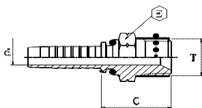
NPTF MALE 60° FLARE
