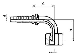
BSP FEMALE 60° FLARE 90° ELBOW WITH O'RING FEMMINA 90° BSP SV.60° CON O'RING 030161
