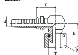
BSP COMPACT FEMALE 60° FLARE 90° ELBOW WITH THRUST WIRE NUT FEMMINA COMPATTA 90° BSP SV. 60° CON DADO SPINATO 030167
